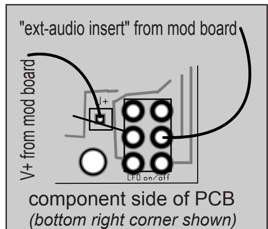
PCB version 2.2a
